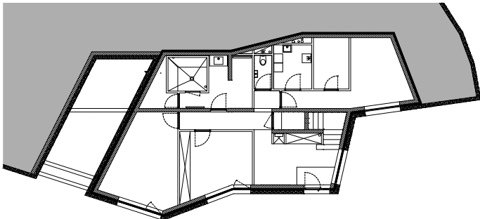
FIRST FLOOR 1:300
