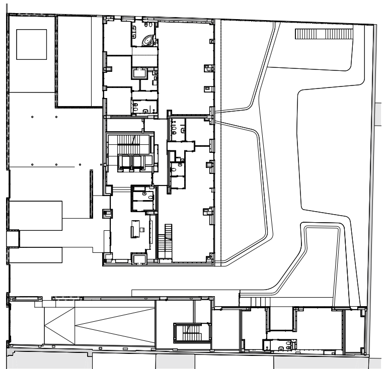
FIRST FLOOR 1:500
