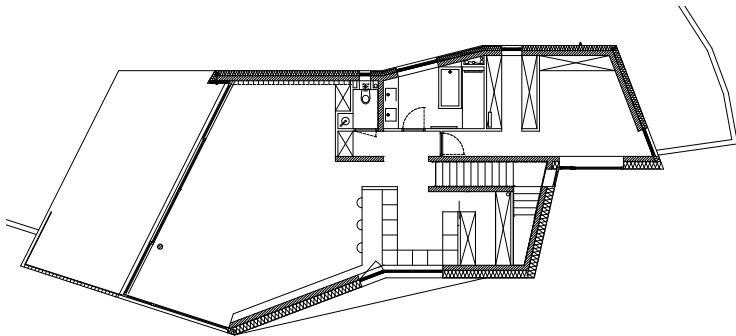
UPPER FLOOR
