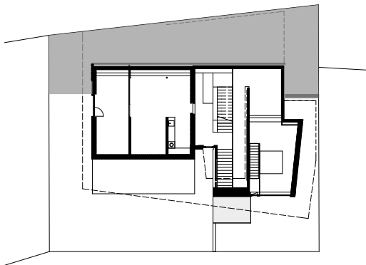
MEZZANINE FLOOR
