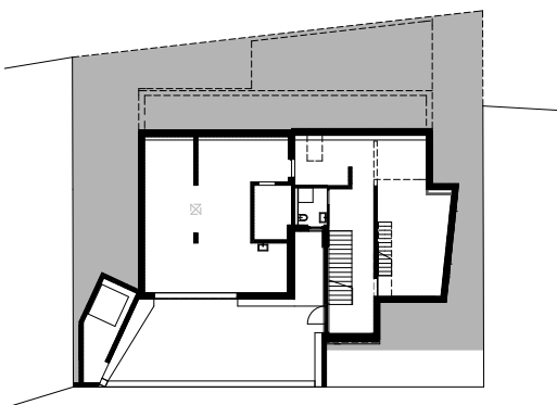
BASEMENT FLOOR 1:500
